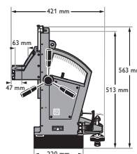
MBS 32 F
