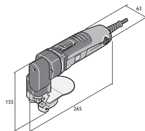
BLS 2.5 E
