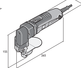
BLS 2.5 E
