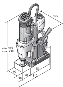
KBM 50 Q
