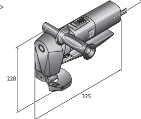
BLS 3.5
