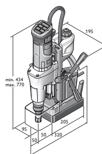
KBM 65 U
