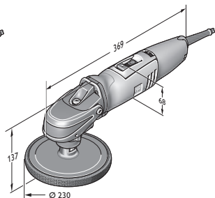
WPO 14-25 E
