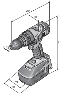
ASB 18 QC
