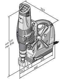
KBM 80 U
