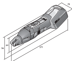
ABSS 18-1.6 E
