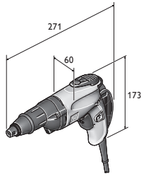
SCT 5-40 X
