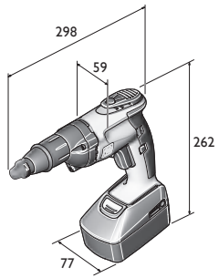
ASCT 18
