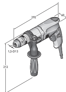
BOP 10-2
