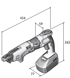
ASCT 18 M
